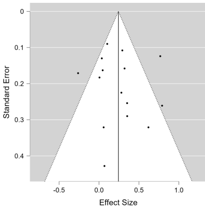
Figure 4 Funnel plot
